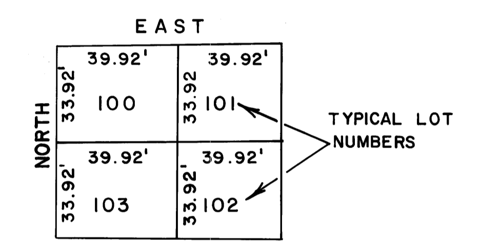
TYPICAL LOT LAYOUT
